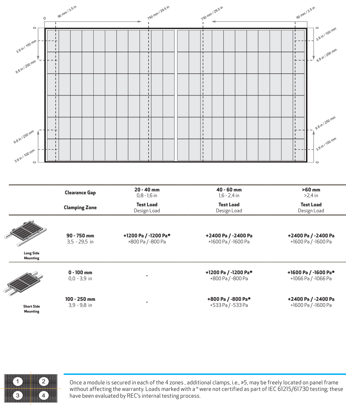
Fig. 2-2 Clamping of REC Alpha Pure 2 panels with Rails parallel to the Long Side of the Panel
