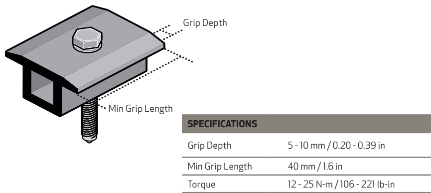
Fig. 1-1 Clamp Specifications
