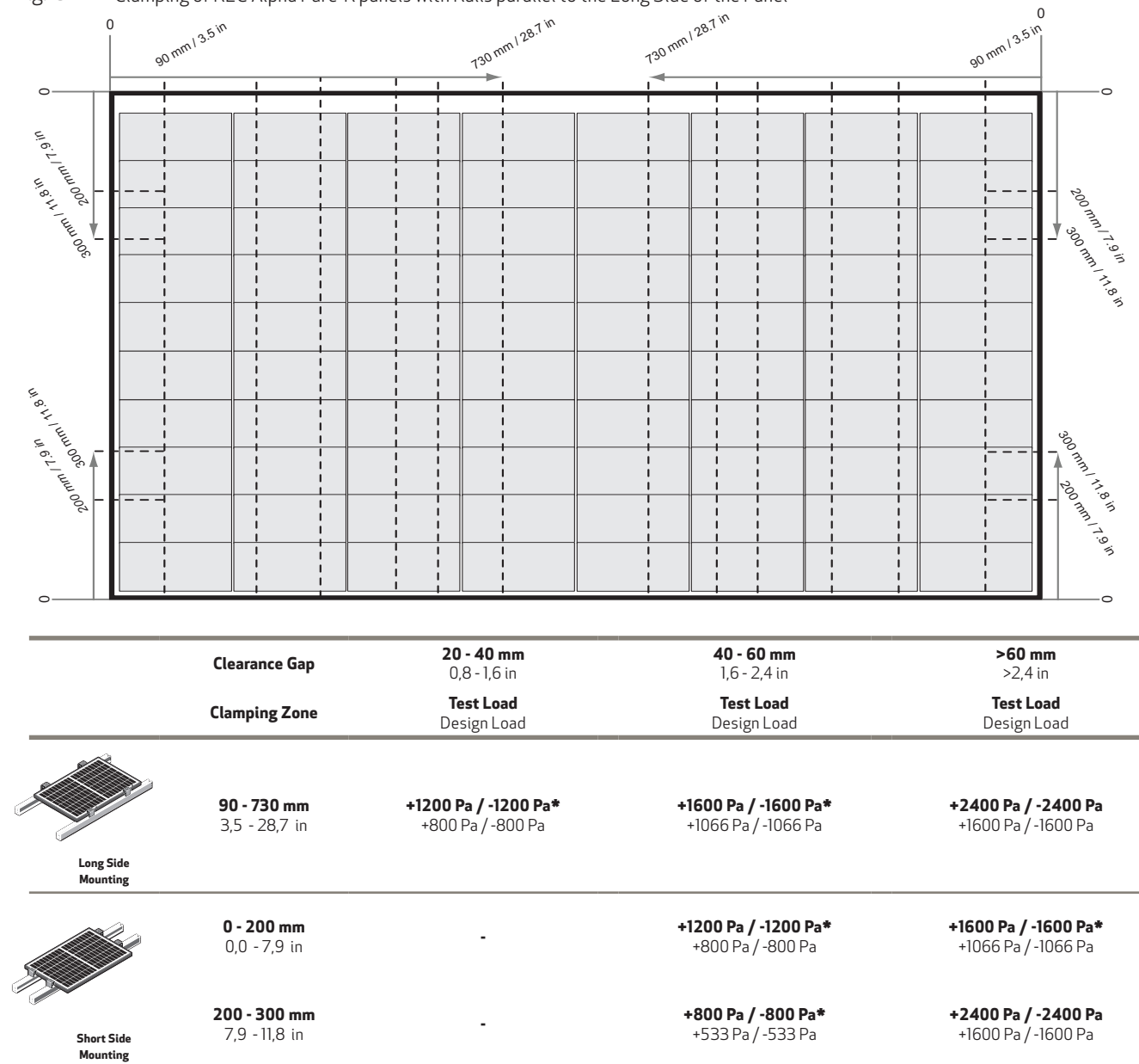
Fig. 3-2 Clamping of REC Alpha Pure-R panels with Rails parallel to the Long Side of the Panel
