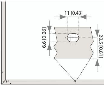
Fig. 12: Mounting holes
