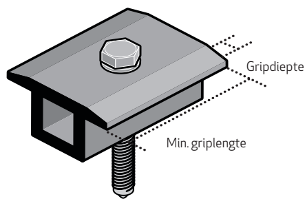
Afb. 1: Klemspecificaties
